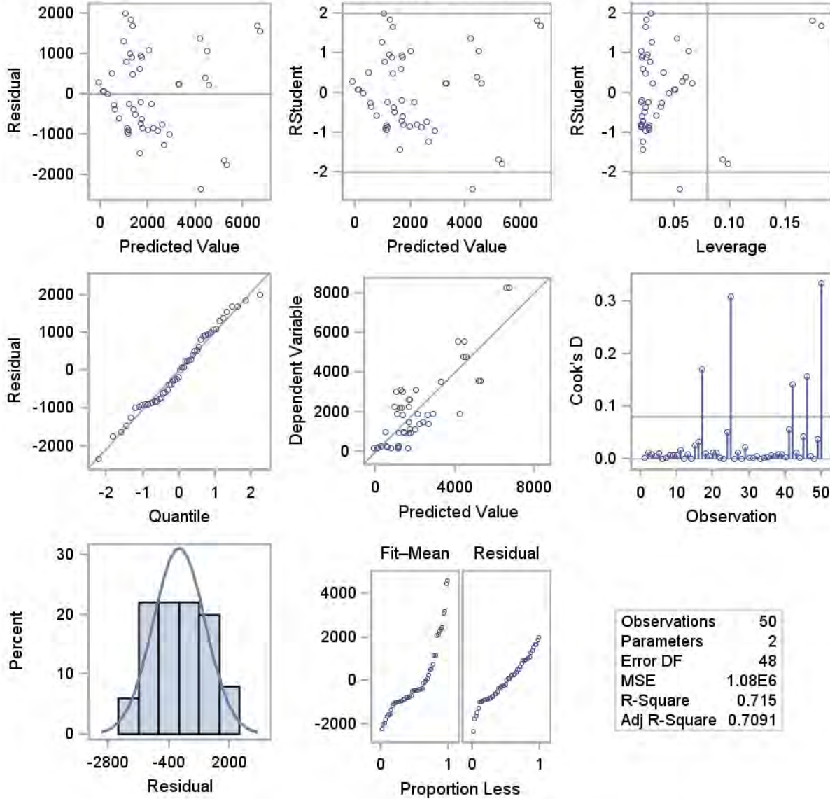
Fit Diagnostics for DepVar
